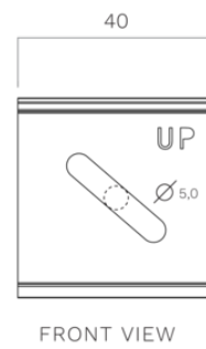
MOUNTING CLIP
